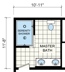
OPTIONAL SERENITY SHOWER
